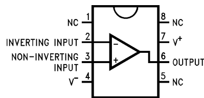
8-Pin DIP/SO
