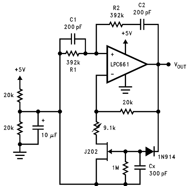
Sine-Wave Oscillator
