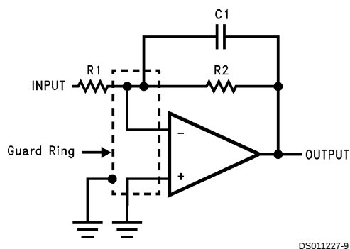
FIGURE 5. Inverting Amplifier Guard Ring Connections
