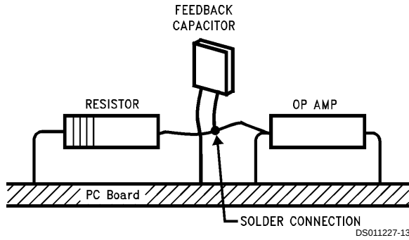
FIGURE 9. Air Wiring
